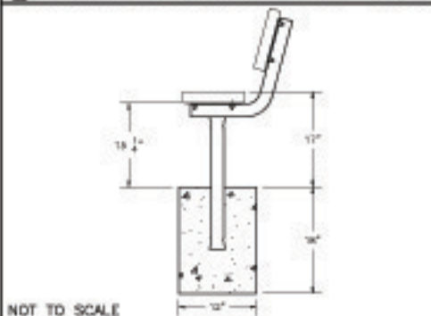
PERMANENT BENCH HEIGHT DETAIL
