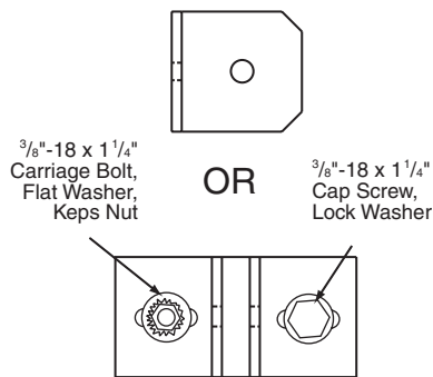
A0315 DUW Short Bank Hangers (for bottom)
