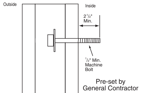
Set-in Bolt
