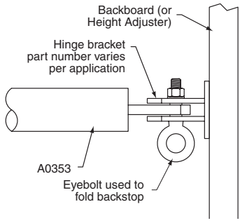
Eye bolt used to fold backstop (DGW).
