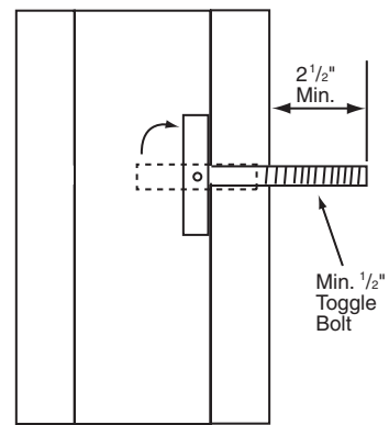
Toggle Bolt
