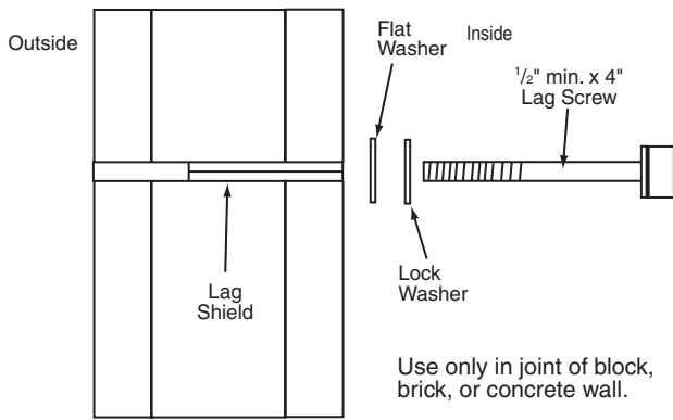
Lag Screw with Lag Shield
