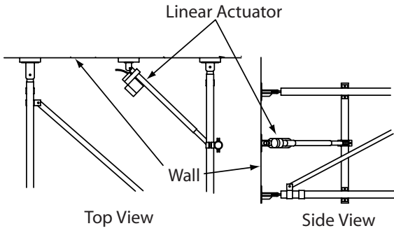
Linear Actuator used to fold backstop (DGW-E).
