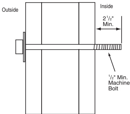
Through Bolt
