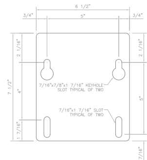
BOLT PATTERN DETAIL
